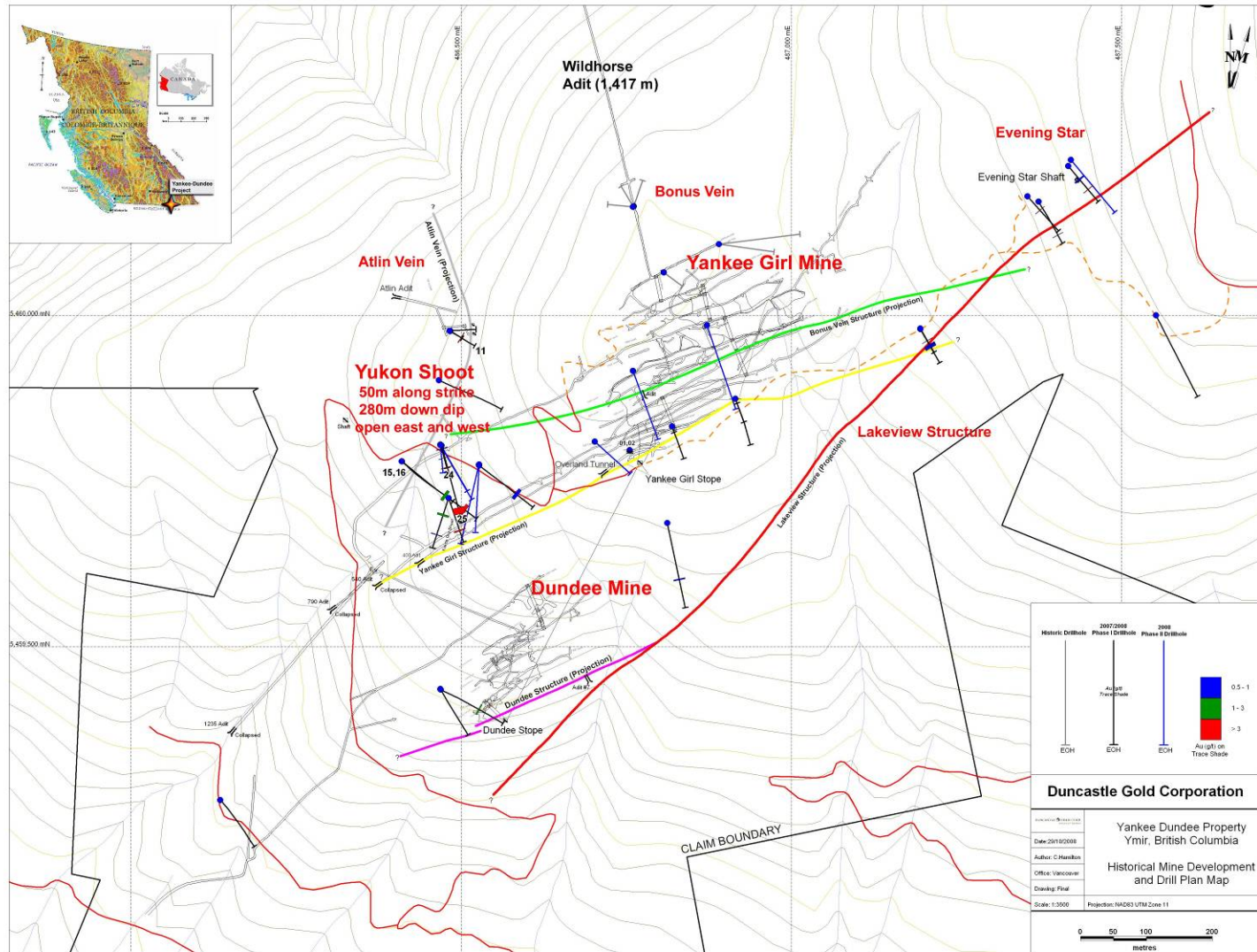
Plan view of historic workings and drill hole locations
